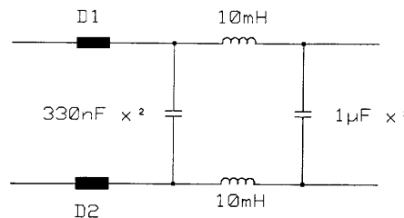
D1/D2=6-Loch-UKW-Breitbanddrossel - D1/D2=6-hole-VHF-wide band choke
