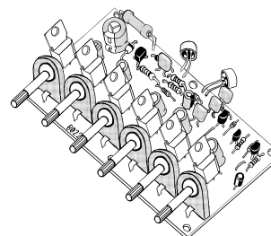
D1/D2=6-Loch-UKW-Breitbanddrossel - D1/D2=6-hole-VHF-wide band choke
